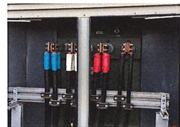
Exposed bushings with 690 V cable terminations inside double doors
